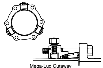
Mega-Lug Cutaway
